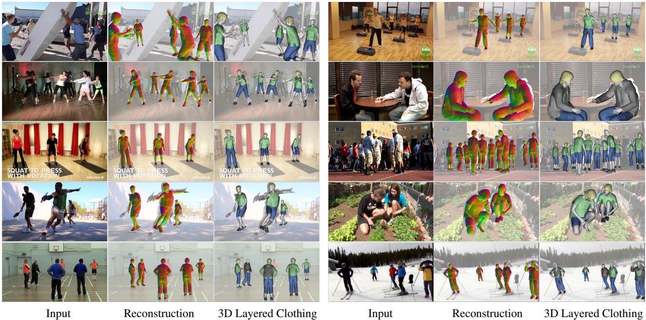
Figure 6: Fitting SMPLicit in multi-person images from the MPII [6] dataset. SMPLicit can dress SMPL with a variety of clothes. Failure case in bottom-right example, where cloth semantic segmentation mixes shirts and jackets in most upper-bodies, and SMPLicit wrongly optimizes two similar intersecting jackets. Best viewed in color with zoom.
